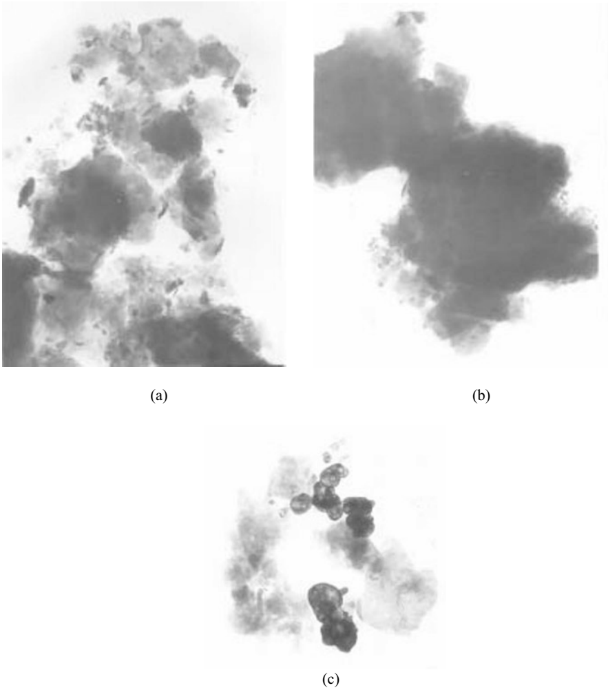
Fig. 5.3 TEM of each grade sediment extracted from Daning sample ( 2 \times 10^4 times): (a) Daning sediment sample; (b) Daning A1; (c) Daning A2
