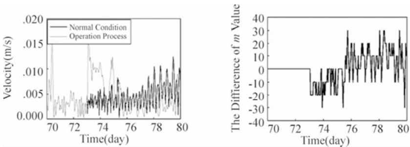
Fig. 7.14 Velocity ( L ) and eutrophication assessment value ( R ) in Daning River mouth (5 m/d)
