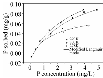
Fig. 5.7 The adsorption isotherm of P on Cuntan sediment at different temperatures
