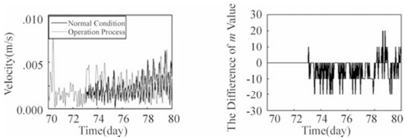
Fig. 7.16 Velocity ( L ) and eutrophication assessment value ( R ) in Xiaojiang River mouth (5 m 3 /5 d)
