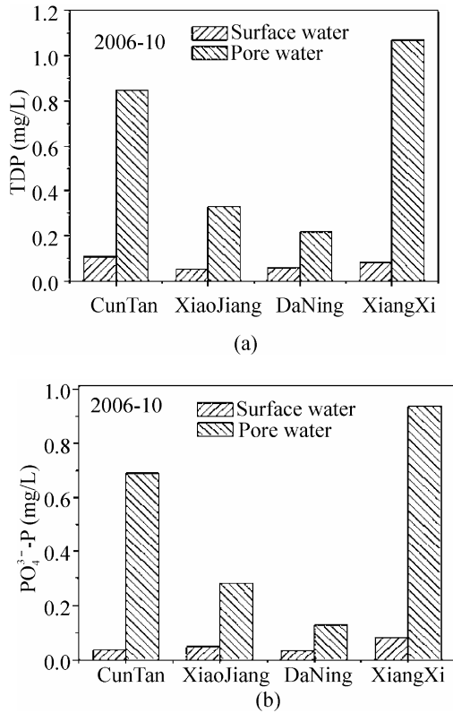
Fig. 2.3 The concentrations of TDP (a) and \text{PO}_4^{3-}\text{-P} (b) in the surface water and pore water from the main tributaries of the Three Gorges Reservoir in 2006
