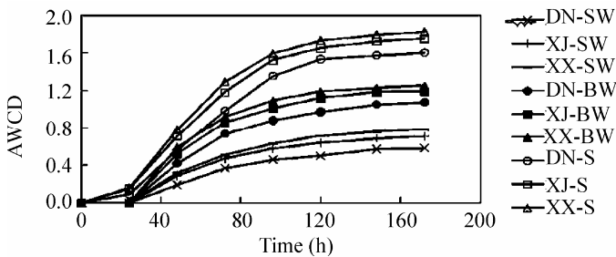
Fig. 7.2 Average well color development (AWCD) of microbial community (DN, Daning River; XJ, Xiaojiang River; XX, Xiangxi River; SW, surface water; BW, bottom water; S, sediment)
