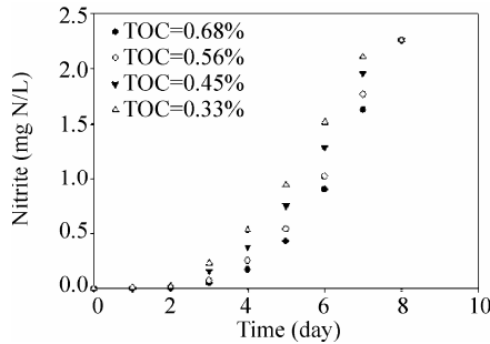
Fig. 4.8 Effect of organic matter contained in suspended particles on the nitrification ( T=28\text{ }^{\circ}\text{C} , sediment concentration=2 g/L, initial \text{NH}_4^+\text{-N} concentrations =2.26 mg/L)
