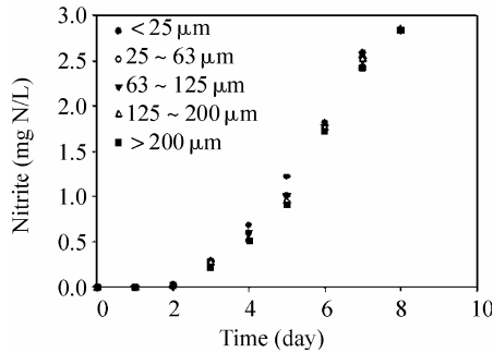
Fig. 4.7 Effect of suspended particle size on the nitrification ( T=28\text{ }^{\circ}\text{C} , sediment concentration=2 g/L, initial \text{NH}_4^+\text{-N} concentrations =2.84 mg/L)
