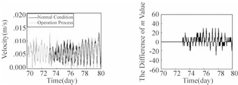
Fig. 7.10 Velocity ( L ) and eutrophication assessment value ( R ) in Xiangxi River mouth (0.5 m/3 h)
