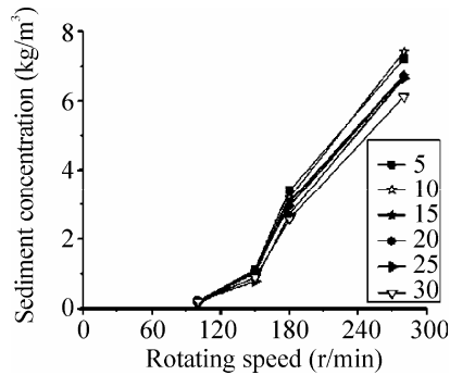
Fig. 3.5 The relationship curve of the sediment concentration and rotating speed of the turbulence-simulation device
