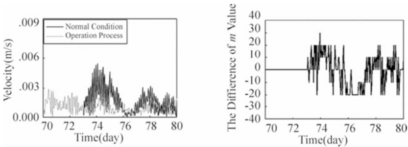
Fig. 7.15 Velocity ( L ) and eutrophication assessment value ( R ) in Meixin River mouth (5 m 3 /d)
